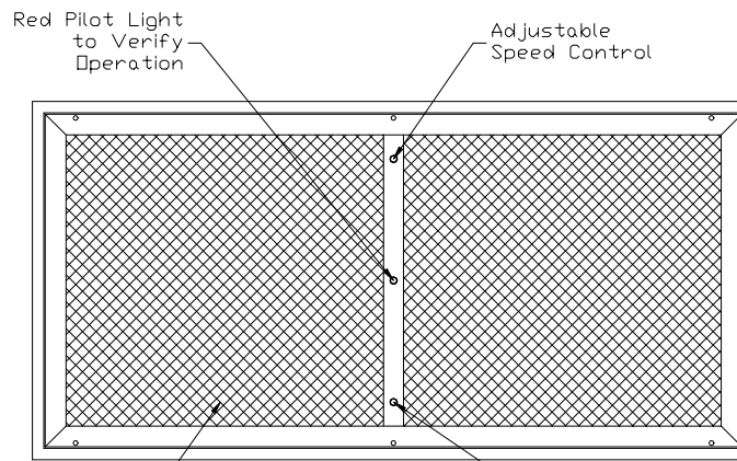
HEPA Filter with Expanded Metal Screen BOTTOM VIEW Challenge Port
