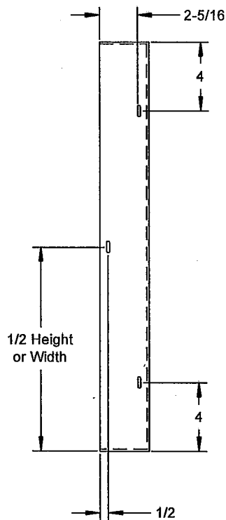
SIDE VIEW Mounting Hole Locations
