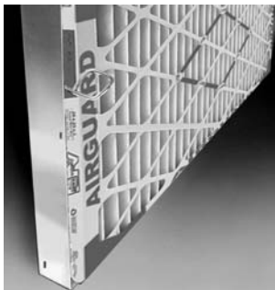
2" Type DP pleated filter installed with RC-1002 2" twist action latch.
