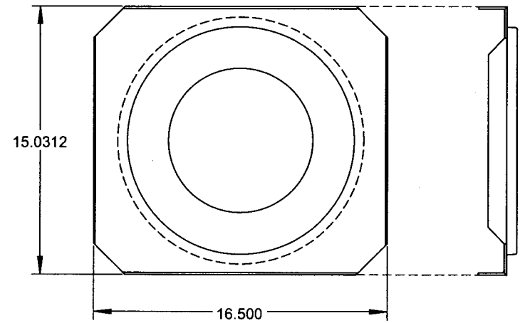
MOUNTING FLANGE DETAIL
